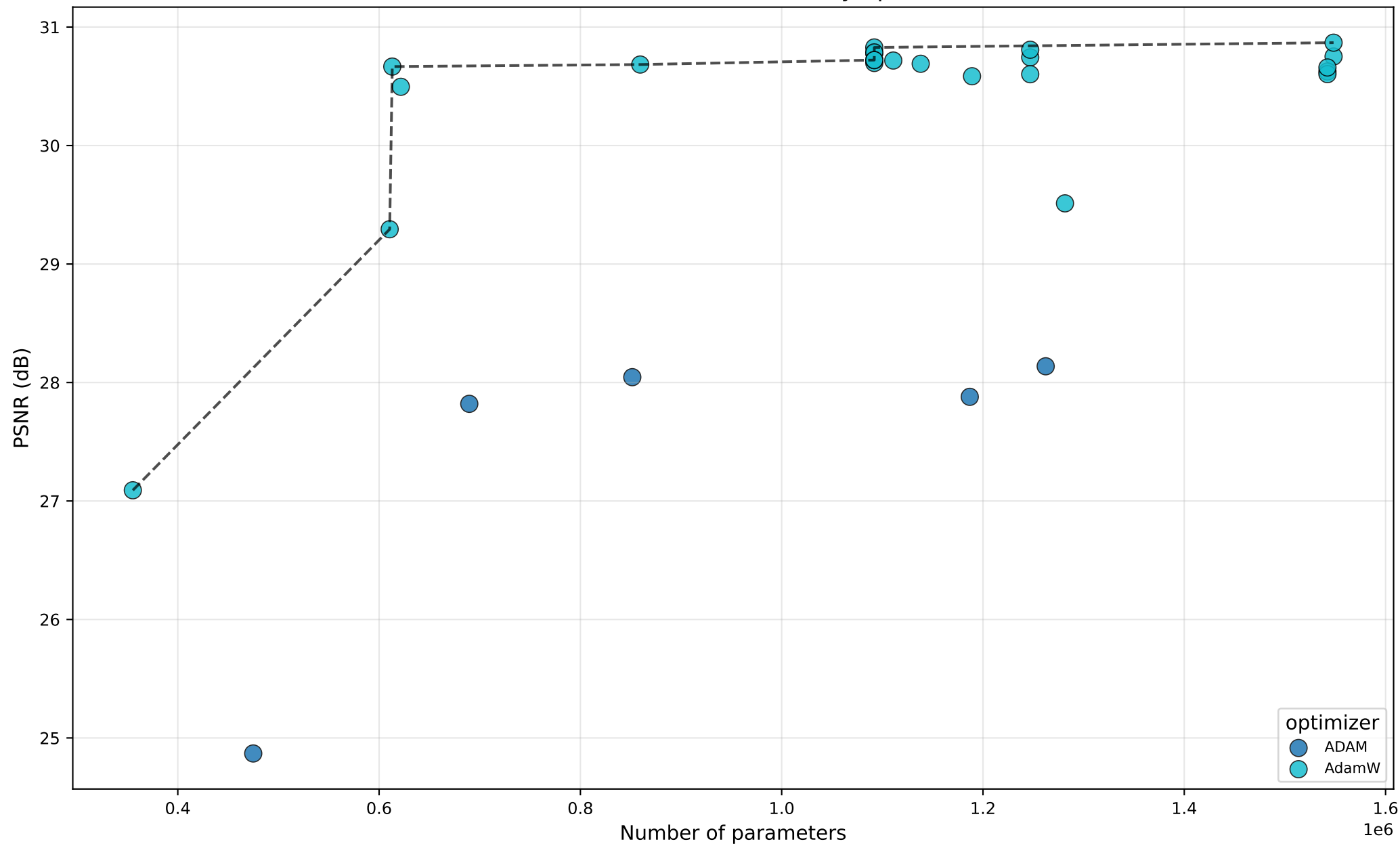
PSNR vs #Params — HAT — by optimizer
